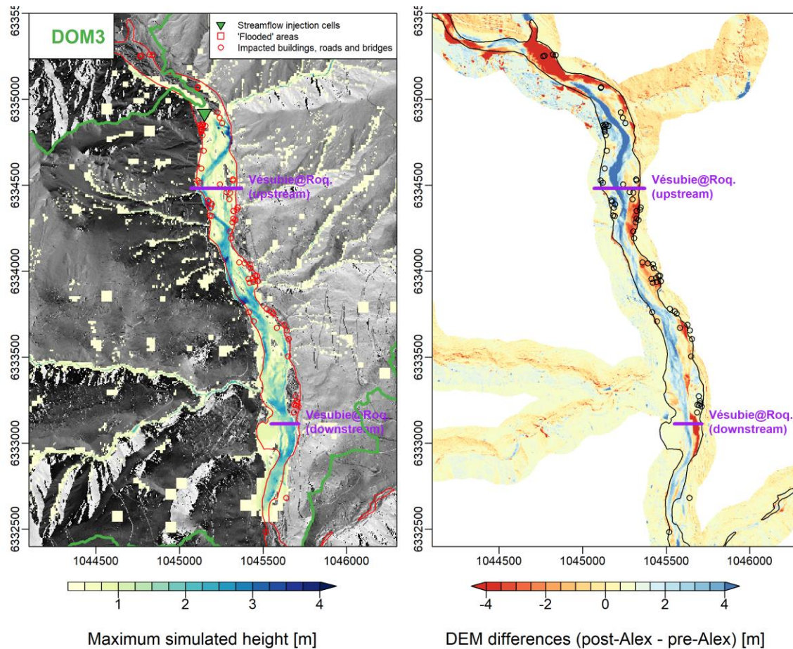
Figure 9: (left) maximum simulated height around Roquebilière, considering the “post-Alex DEM” and the DOM3 simulation configurations (only the cells with more than 40 [cm] of water are highlighted here); (right) DEM differences for Roquebilière area.
