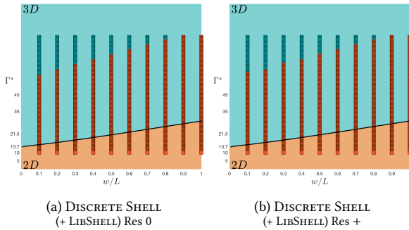
Fig. 10. Detailed results of the Lateral Buckling test for DISCRETE SHELL and our two different mesh resolutions up to \Gamma^* = 80 .
