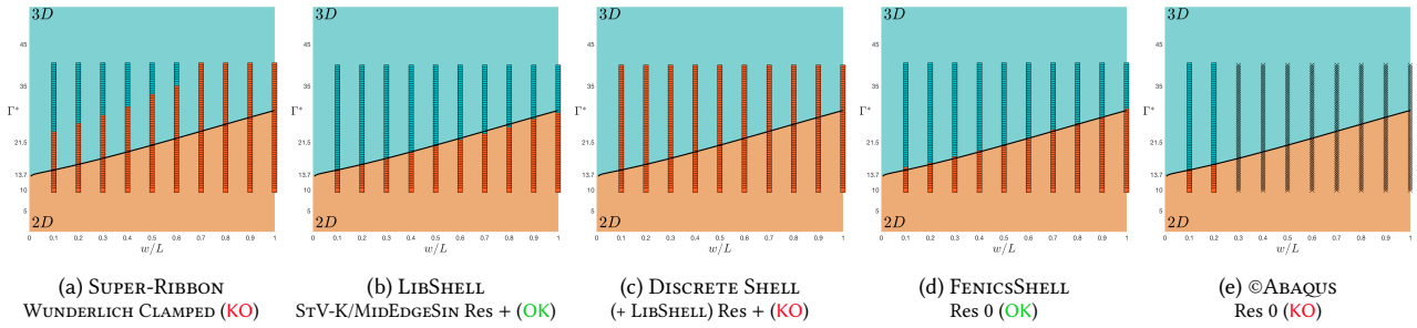
Fig. 9. Results of the Lateral Buckling test.
