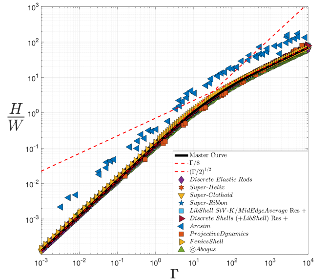
Fig. 6. Results on the Cantilever test.
