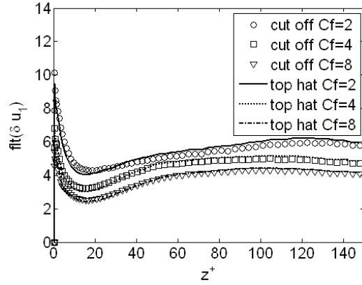
Figure 22. Flatness of the correction term component in the streamwise direction as a function of z^+ . St=5 .
