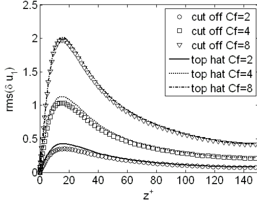
Figure 16. R.m.s. values of the correction term component in the streamwise direction as a function of z^+ . St=5 .
