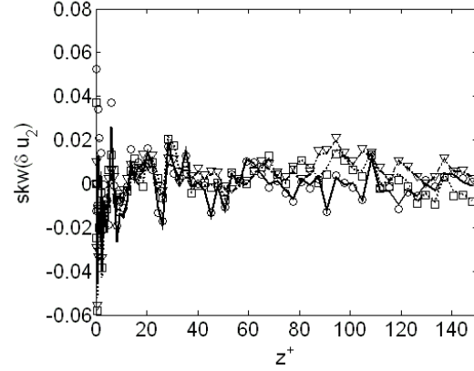
Figure 20. Skewness of the correction term component in the spanwise direction as a function of z^+ . St=5 .
