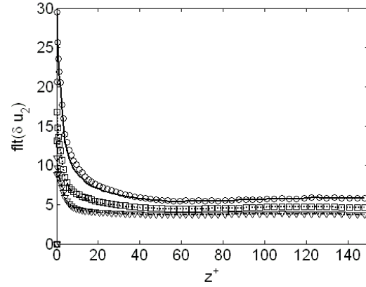
Figure 23. Flatness of the correction term component in the spanwise direction as a function of z^+ . St=5 .
