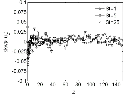
Figure 9. Skewness of the SGS velocity correction component in the spanwise direction as a function of z^+ . Cut-off filter with CF=4.
