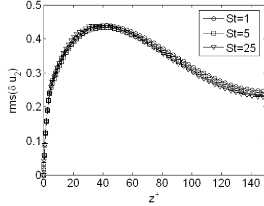
Figure 6. R.m.s values of the SGS velocity correction component in the spanwise direction as a function of z^+ . Cut-off filter with CF=4.
