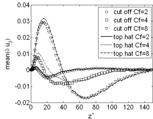
Figure 15. Mean values of the correction term component in the wall-normal direction as a function of z^+ . St=5.
