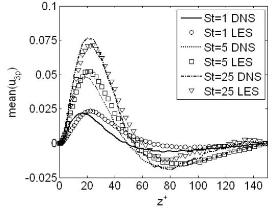
Figure 4. Effects of filtering on the fluid mean normal velocity seen by the particles. Cut-off filter with CF=4.
