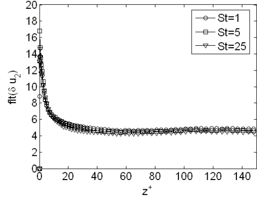
Figure 12. Flatness of the SGS velocity correction component in the spanwise direction as a function of z^+ . Cut-off filter with CF=4.
