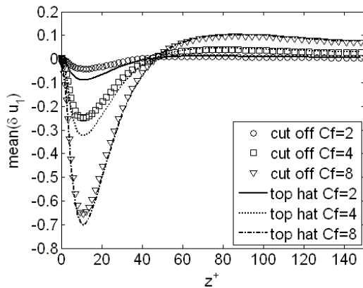
Figure 14. Mean values of the correction term component in the streamwise direction as a function of z^+ . St=5.
