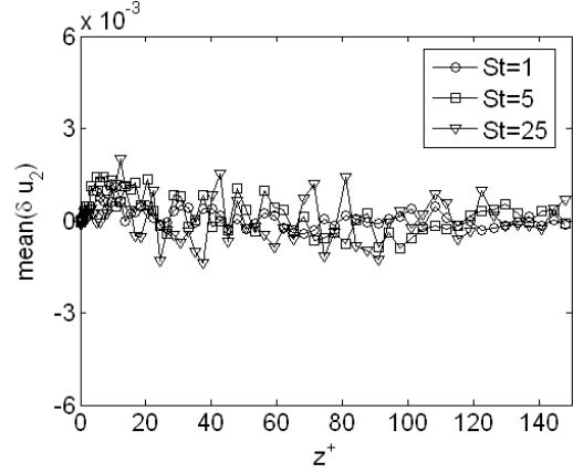
Figure 2. Mean values of the SGS velocity correction component in the spanwise direction as a function of z^+ . Cut-off filter with CF=4.
