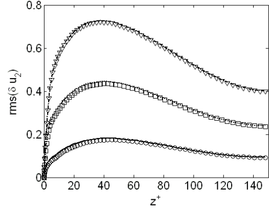
Figure 17. R.m.s. values of the correction term component in the spanwise direction as a function of z^+ . St=5 .
