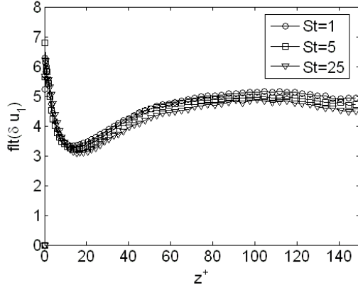
Figure 11. Flatness of the SGS velocity correction component in the streamwise direction as a function of z^+ . Cut-off filter with CF=4.
