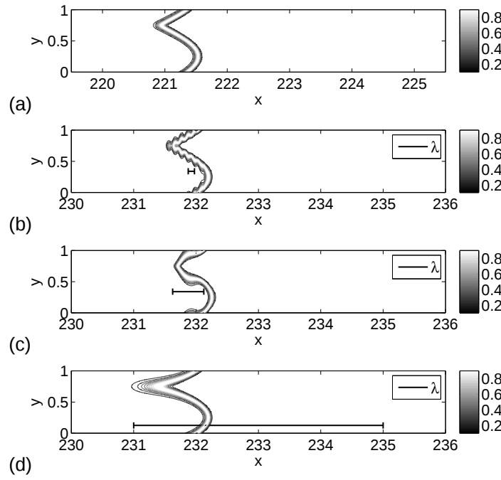
Figure 2: Snapshot of 4\theta(1-\theta) for a fixed Peclet number ( Pe = 100 ) and for Damköhler number Da = 100 . Panel (a) refers to a incompressible simulation ( \epsilon = 0 ) while for the others \epsilon = 0.5 . For the compressible tests the characteristic length \lambda is set to be approximately lower (panel (b), \lambda = 0.1 ), between (panel (c), \lambda = 0.5 ) or greater (panel (d), \lambda = 4 ) than the two thicknesses \Delta and \delta .
