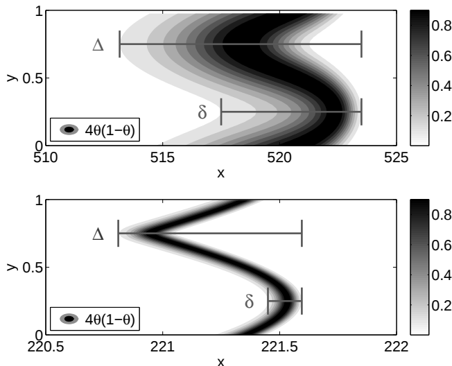
Figure 1: Shape of the active part of the front (we use the function 4\theta(1 - \theta) , which is maximal for \theta = 0.5 ), for a fixed Peclet number ( Pe = 100 ) and for two different reaction rates. Taking as reference the incompressible test case ( \epsilon = 0 ) we can define two different thicknesses. The bare front thickness as \delta \sim \sqrt{D/\alpha} and the distance between the tip and the tail of the reacting region \Delta . For a slow reaction (upper panel, Da = 1 ), we have approximately \Delta \approx 10 and \delta \approx 6 . For fast reaction (lower panel, Da = 100 ) \Delta \approx 0.8 and \delta \approx 0.15 .
