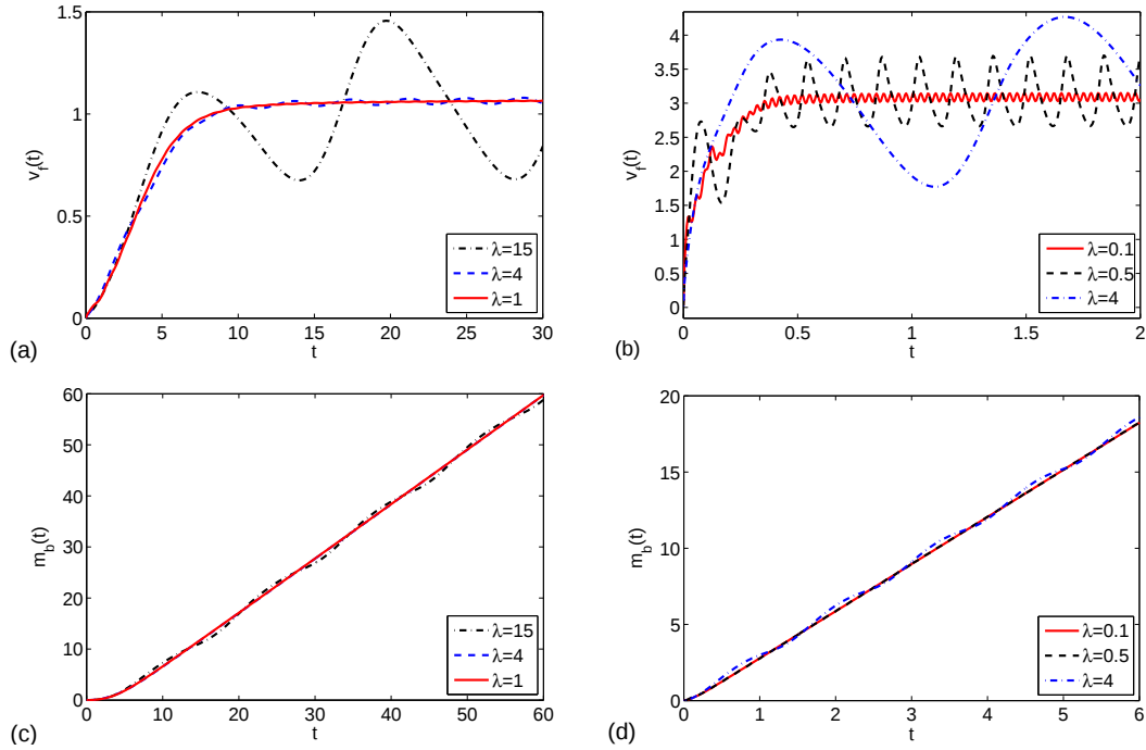
Figure 3: (Color online) Front speed and burnt mass ( m_b(t) = \int_0^t v_f(t) dt ) as function of time for a fixed Pe = 100 , two different Damköhler ( Da = 1 in panel: a,c ; Da = 100 in panel: b,d) and different \lambda .
