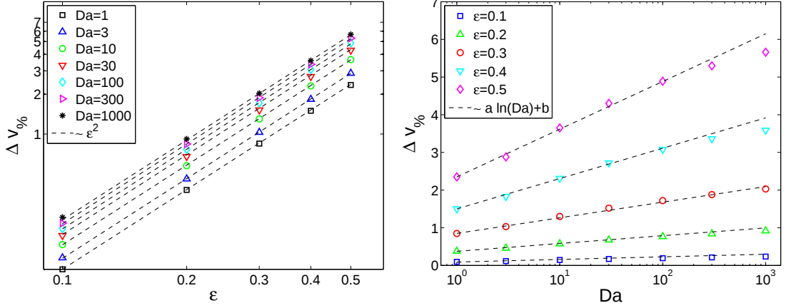
Figure 4: (Color online) Comparison of the front speed between compressible and incompressible shear flow for a fixed Peclet number ( Pe = 100 ) at different compressibility magnitude \epsilon (on the left) and for different Damköhler (on the right).
