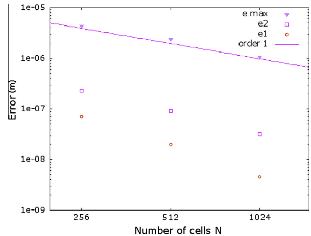
Fig. 3. Error norms defined in Eqs. (16)–(18) with respect to the number of cells of the simulation calculated for the case “ I = 25 \text{ mm h}^{-1} and S_0 = 5\% ” for the Darcy–Weisbach friction term. Results shown in log–log scale. The straight line is a guide for the eyes of an order 1 curve.
