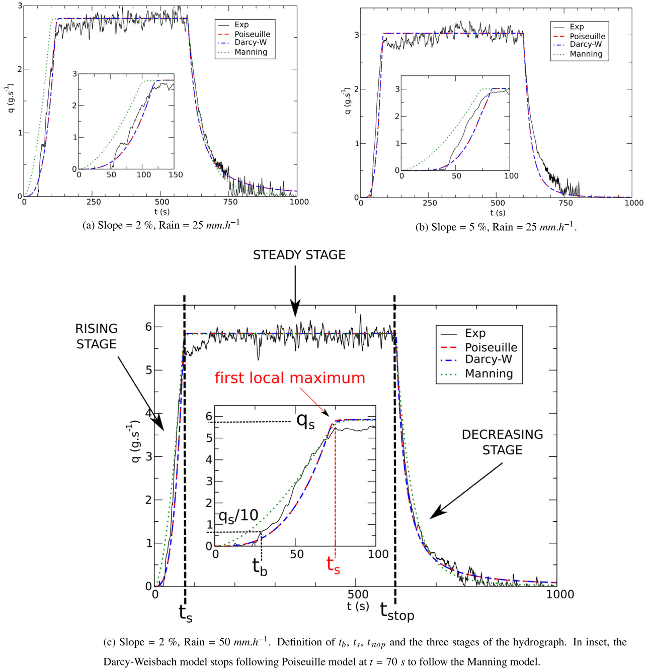
Fig. 4. Numerical results with different friction terms and experimental discharge at the end of the slope versus time for different slopes and rain intensities. Zoom of the rising limb in inset.
