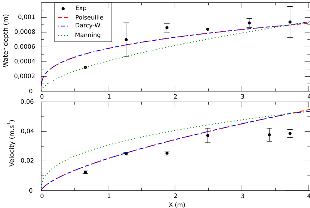
Fig. 5. Water depth (top) and velocity (bottom) profiles along the slope at the steady stage ( t = 599 s). Error bars are standard errors.
