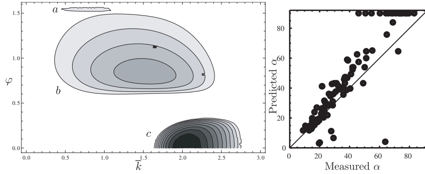
FIGURE 3. Left: Growth rate Im(\bar{\omega}) of the three-dimensional instabilities of a granular bed submitted to erosion by a laminar flow, as a function of the wave-vector norm k , and angle \phi with respect to the x direction. The blank domain corresponds to negative values of the growth rate, that is, stable modes. In this typical example, three types of instabilities of different geometrical characteristics can develop: (a) longitudinal striation, which maximum growth rate lies at angle close to \pi/2 ; (b) bar instability, which can occur at any value of the angle \phi ; (c) ripple instability, which crests are perpendicular to the main flow direction, that is, \phi = 0 . The bar instability is probably responsible for the initiation of rhomboid patterns. In this example, the parameters have values Fr = 0.90 , S = 0.015 , Bo = 2.77 and \Theta = 0.448 . Right: Comparison between the three-dimensional model of the present paper, and the experimental results of Devauchelle et al. [5]. The comparison concerns the geometrical characteristics of the rhomboid pattern: opening angle \alpha = \pi/2 - \phi (in degrees).
