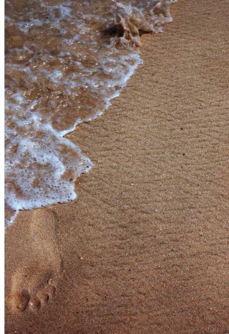
FIGURE 1. Typical sea shore diamond-shaped erosion patterns
