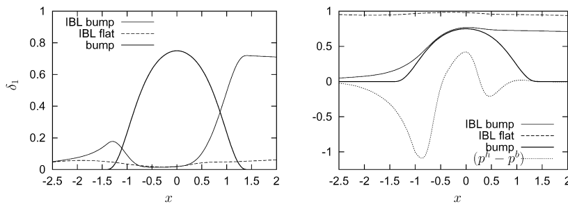
Fig. 8. Left: the displacement functions \delta_1^b (IBL bump) and \delta_1^h (IBL flat). A large value of \delta_1 is associated to boundary layer separation. A thin value is associated to the large acceleration at the throat. Right: the difference of pressure p^h - p^b is plotted, the “final effective” channel is plotted: 1 - \delta_1^h and f_b + \delta_1^b ; the jet due to separation is visible.
