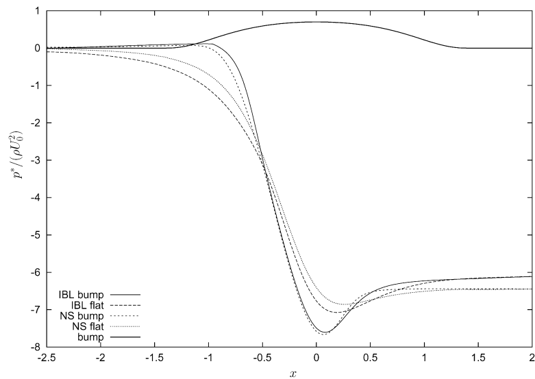
Fig. 6. Comparison of integral IBL and NS pressures. The IBL approach well predicts the over pressure on the flat wall and the positions of the minima of the pressures after the throat.
