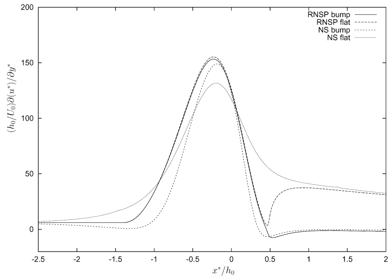
Fig. 5. Comparison of RNSP and NS wall shear stress. The flat wall shear stress is over predicted by RNSP at the maximum, but in the wake ( x^*/h_0 > 1 ) it is better.
