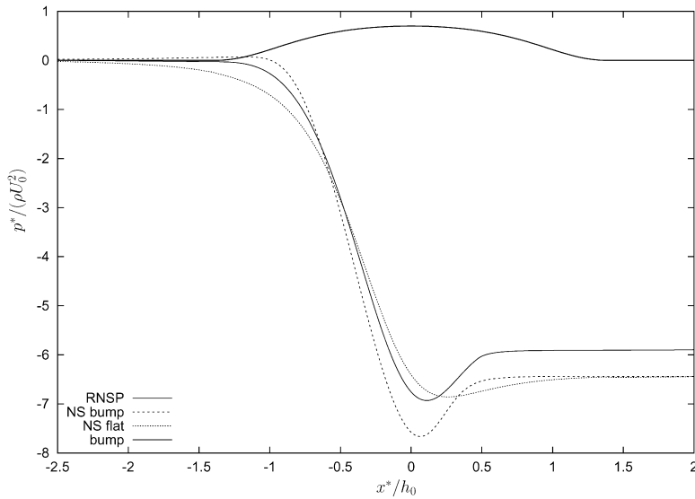
Fig. 4. Comparison of RNSP and NS pressures, RNSP solution is an approximation of the two NS pressures. The geometry is plotted as well.
