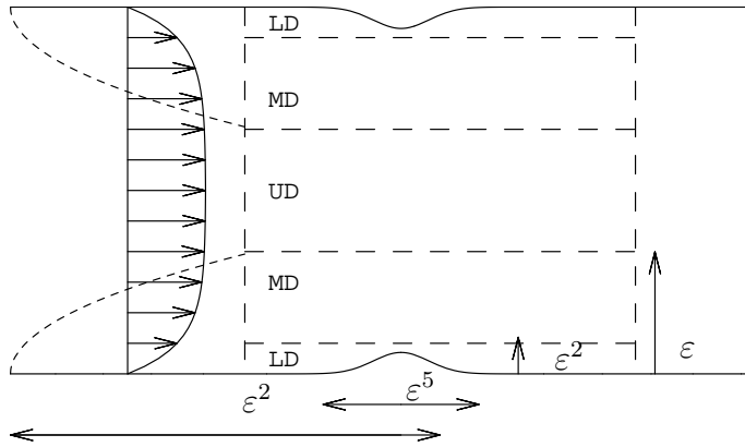
Fig. 8. Flow configuration in the Triple Deck case : A mild constriction, of length \varepsilon^5 and height \varepsilon^2 , is located at station \varepsilon^2 , lying in the lower deck (LD). This thin layer is included in the boundary layer of thickness \varepsilon , or main deck (MD). The upper deck (UD) is the inviscid core.
