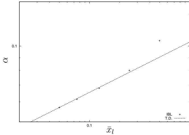
Fig. 10. Incipient separation : comparison between Triple Deck and IBL : value of \alpha that promotes the incipient separation versus the longitudinal width of the constriction \bar{x}_l computed by the full IBL equations. The line of slope 1/5 ( i.e. \alpha \simeq \bar{x}_l^{1/5} ) is the Triple Deck prediction.
