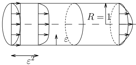
Fig. 3. Unstricted situation : entry problem. Starting from a flat velocity profile, a Poiseuille profile is obtained at the exit, i.e. at a distance O(1) in the R_0 Re scale. Near the entrance, i.e. at a distance O(\varepsilon^2) , the IBL formulation is valid : the boundary layer thickness is of order O(\varepsilon) in the R_0 scale.
