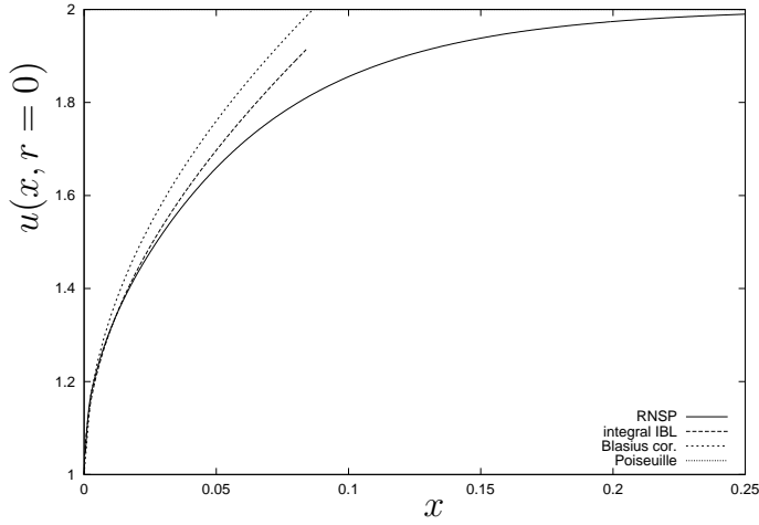
Fig. 4. Unconstricted situation : longitudinal evolution of the velocity at the centre of the pipe. RNSP : numerical solution of the RNSP equations ; integral IBL : solution obtained with the integral IBL approach, rescaled in the x variable ; "Blasius cor." : first order correction ( u = 1 + 3.4x^{1/2} ) to the Blasius solution (which is u = 1 ), as obtained in §3.2.5. Note that the Poiseuille value is independent of x and equals 2.
