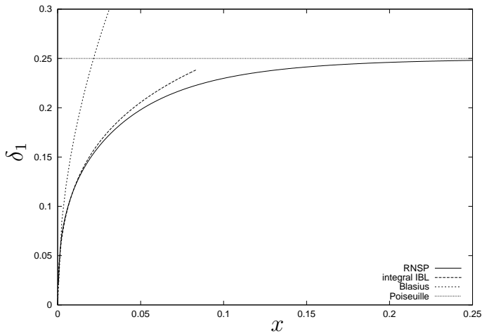
Fig. 6. Unconstricted situation : longitudinal evolution of the displacement thickness. RNSP : numerical solution of the RNSP equations ; integral IBL : solution obtained with the integral IBL approach, rescaled in the x variable ; Poiseuille : \delta_1 = 1/4 ; Blasius : \delta_1 = 1.7\bar{x}^{1/2} .
