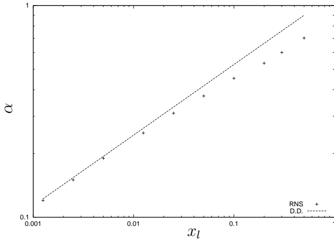
Fig. 13. Incipient separation : comparison between Double Deck and RNSP : value of \alpha which promotes the incipient separation versus the longitudinal width of the constriction x_l computed by the RNSP approach. The line of slope 1/3 ( i.e. \alpha \simeq x_l^{1/3} ) is the Double Deck prediction.
