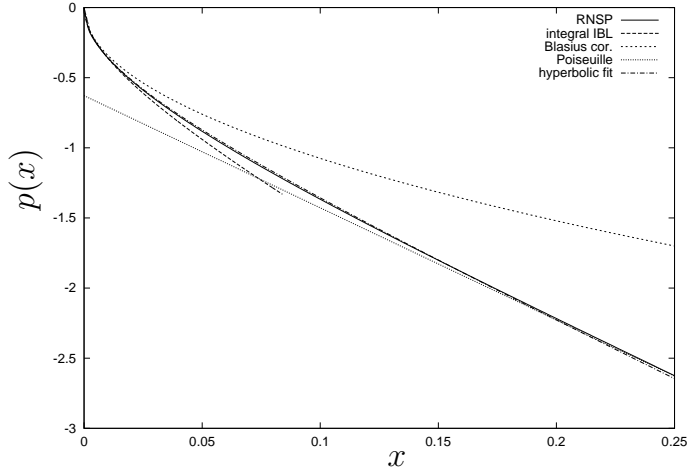
Fig. 5. Unconstricted situation : longitudinal evolution of the pressure : RNSP : numerical solution of the RNSP equations ; integral IBL : solution obtained with the integral IBL approach, rescaled in the x variable ; Poiseuille : p = -0.63 - 8x , see §3.1 ; Blasius cor. : first order correction ( -2\varepsilon\bar{\delta}_{1Blasius} ) to the Blasius solution (which is p = 0 ), as obtained in §3.2.5 ; hyperbolic fit : ad hoc fitting relation (Eq. 20).
