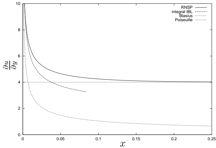
Fig. 7. Unconstricted situation : longitudinal evolution of the WSS. RNSP : numerical solution of the RNSP equations ; integral IBL : solution obtained with the integral IBL approach, rescaled in the x variable ; Poiseuille : \tau = 4 ; Blasius : \tau = 0.33x^{-1/2} .
