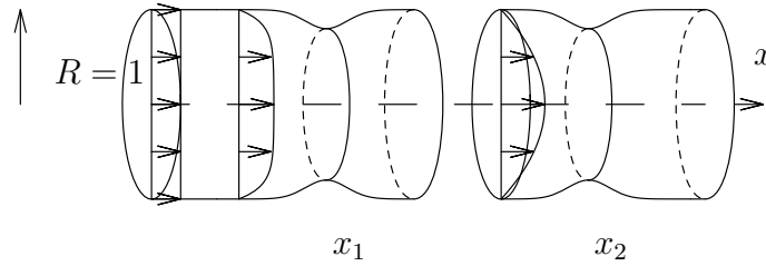
Fig. 2. Flow configurations : A constriction may be located at station x_1 where an inviscid fluid core still exists, see §3.2.1: IBL or §3.3: Triple Deck (Fig. 8), or at station x_2 where the Poiseuille profile has developed, see §3.4: Double Deck (Fig. 11). If the constriction is short but severe enough, the exact entrance velocity profile has no importance, see §3.6.1: IBL.
