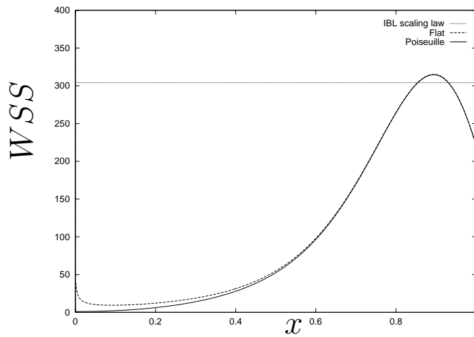
Fig. 16. Longitudinal evolution of the WSS along the convergent part of a 70% stenosis computed using the RNSP approach with Re = 500 ; solid line: Poiseuille entry profile ; broken line: flat entry profile.
