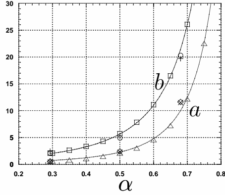
Fig. 14. Coefficient a and b for the maximum WSS (see Eq. 43). \diamond : coefficient a derived from Siegel for \lambda = 3 ; \times : coefficient a derived from Siegel for \lambda = 6 ; \circ : coefficient b derived from Siegel for \lambda = 3 ; + : coefficient b derived from Siegel for \lambda = 6 . Coefficients a ( \triangle ) and b ( \square ) obtained using the IBL integral method ; solid lines : Coefficients a and b from Eq. 44.
