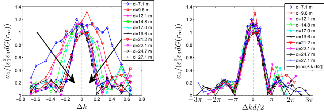
FIGURE 7. Rescaled amplitude a_4/(\varepsilon_1^2 \varepsilon_3 dG(r_m)) measured at different distances d for out-of-resonance conditions ( \varepsilon_1 = \varepsilon_3 = 0.07 and f_1 = 0.9 Hz.). Left: rescaled a_4 vs detuning \Delta k . Symbols corresponds to different d = 7 up to 27 m (see arrows). Right: rescaled a_4 vs normalized detuning \Delta kd/2 . Solid line: absolute sinc function |\text{sinc}(\Delta kd/2)| from Longuet-Higgins (1962) estimation or from equation (3.5).
