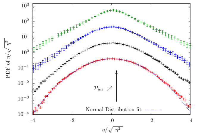
FIG. 5. (Color online) Probability density functions of the large-scale wave height for the spectra reported in Fig 4 (same color-key). Data and errorbars are multiplied by \times 1 , \times 10 , \times 100 and \times 1000 for clarity.
