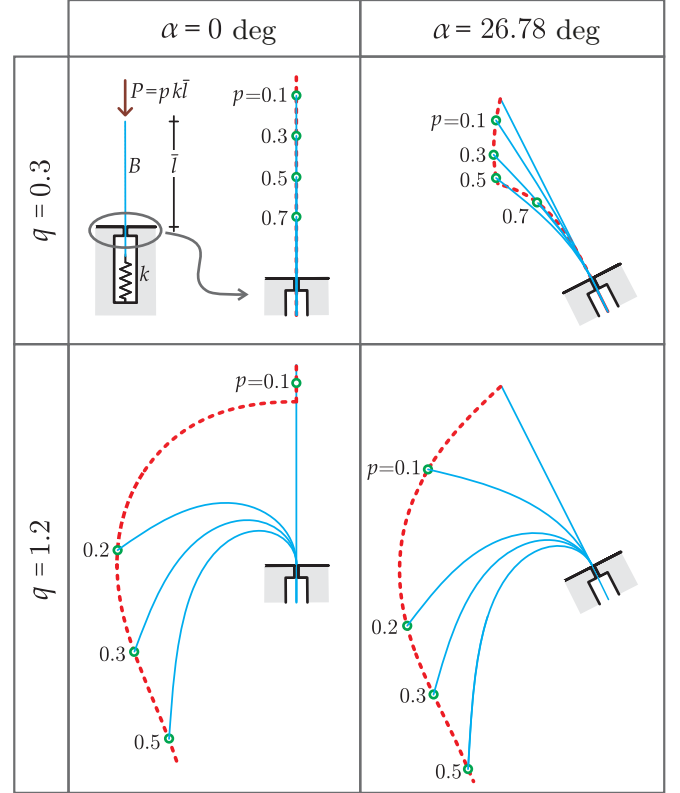
FIG. 2. Trajectories (red dashed curves) traced by the loaded end of the rod during a monotonic loading, for stiffness ratios q = 0.3 (upper part) and q = 1.2 (lower part), with q = 16k\hat{l}^3/(27\pi^2 B) . Intermediate deformed configurations (blue curves) are displayed for specific normalized loads p = P/(k\hat{l}) . The behavior of the imperfect ( \alpha = 26.78^\circ , right) system shows that ‘‘asymptotic self-restabilization’’ can occur only when the perfect system ( \alpha = 0 , left) does not suffer buckling.
