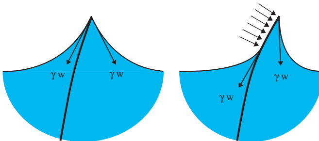
Fig. 12. The two different types of configurations of lightly deflected states at non-zero L_c . Left: the two menisci joining the apex of the beam to the asymptotical bath height H are vertically symmetric. Right: the beam has a semi-submerged part.
