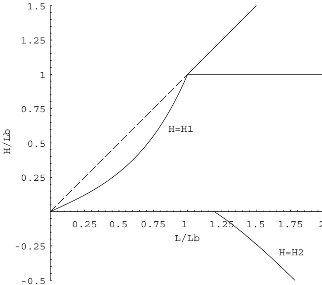
Fig. 9. Extended version of Fig. 7 with the new curve H = H_2(L/L_b) where diving states lose stability as the end of the beam detaches from the interface.
