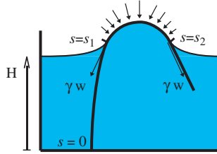
Fig. 10. A lying configuration: at s = s_1 and s = s_2 , the interaction with the surface is modelled by discrete jumps in the inner force vector \mathbf{n}(s) . In the region s_1 < s < s_2 , the hydrostatic pressure yields a distributed force that is continuously changing \mathbf{n}(s) .
