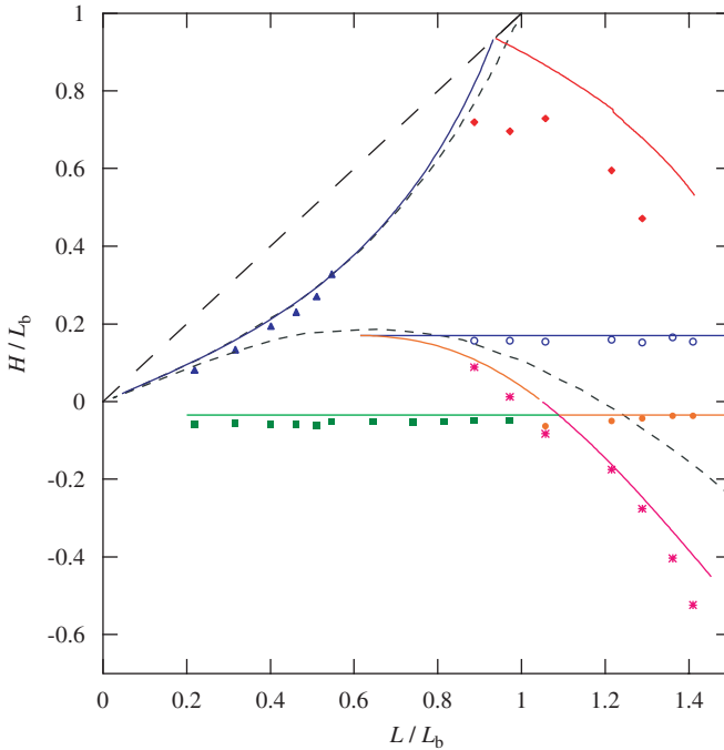
Fig. 19. Experimental and numerical phase diagram for a fibre with a radius of 18\ \mu\text{m} ( L_b = 9.8\ \text{cm} ). Experimental data are plotted as symbols, whereas numerical curves are in continuous line (with gravity) or dotted lines (without gravity).
