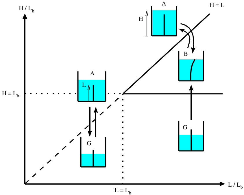
Fig. 5. Parameter regimes for the buckling of a straight beam, of length L , by surface tension. Short beams ( L < L_b ) pierce the liquid interface, whereas longer beams are deflected.
