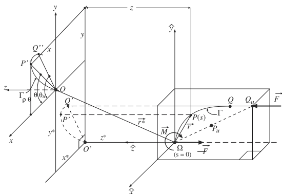
Fig. 1 Elastica \Gamma in space of a thin compressed rod; \vec{r}^* auxiliary vector to be added to \vec{r} ; Oxyz , final three-orthogonal frame of reference; \rho and \theta polar coordinates superimposed upon the cartesian plane xOy on which \Gamma is projected as \Gamma_{\rho\theta}
