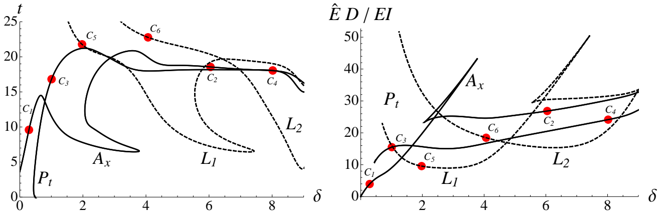
Figure 5: Post-buckling paths: (Left) Force-displacement curves for f_\gamma = 20 , where t is the applied tension and \delta the end-shortening, and (Right) Energy \hat{E} as function of \delta . Solid lines represents both A_x configurations, where the beam shape is symmetric with respect to the axis joining the center of the disk (x_C, y_C) and the beam midpoint (x(\ell/2), y(\ell/2)) , and P_t configurations, where the beam shape is symmetric with respect to the beam midpoint P_t . Dashed lines correspond to L_1 and L_2 configurations.
