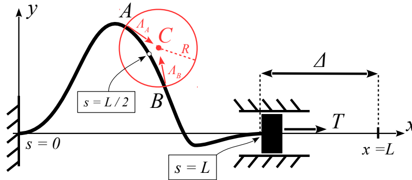
Figure 2: An elastic beam held in tension at its extremities, and buckling under the action of compressive forces at a disk. The beam is clamped at both ends. The deformation of the beam is described by the angle \theta(S) between the tangent to the beam and the x -axis, where S \in [0, L] is the arc-length along the beam.
