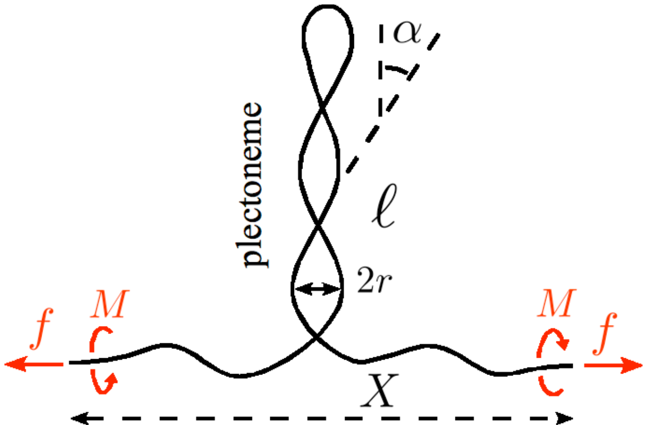
FIG. 1: Supercoiled DNA under force and torque. Molecule length is partitioned between two “phases”: an extended phase, and a plectonemic phase where strong self-interaction occurs.
