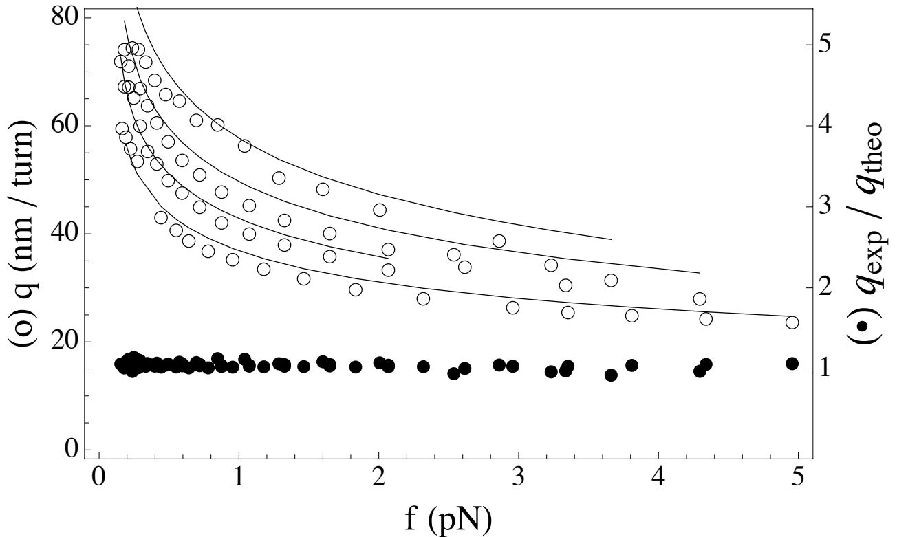
FIG. 2: Comparison of experimental and theoretical slopes as function of the applied force, for 50, 100, 200, and 500 mM salt (top to bottom): (a) experimental data from Ref. [1] (circles); (b) theoretical solution of the full equations \nabla\mathcal{G} = \mathbf{0} (continuous lines); (c) ratio of the experimental slopes to the formula in Eq. (16) (filled circles). Experimentally given values of A/kT = 46, 47, 44, 45 nm and C/kT = 94 nm were used.
